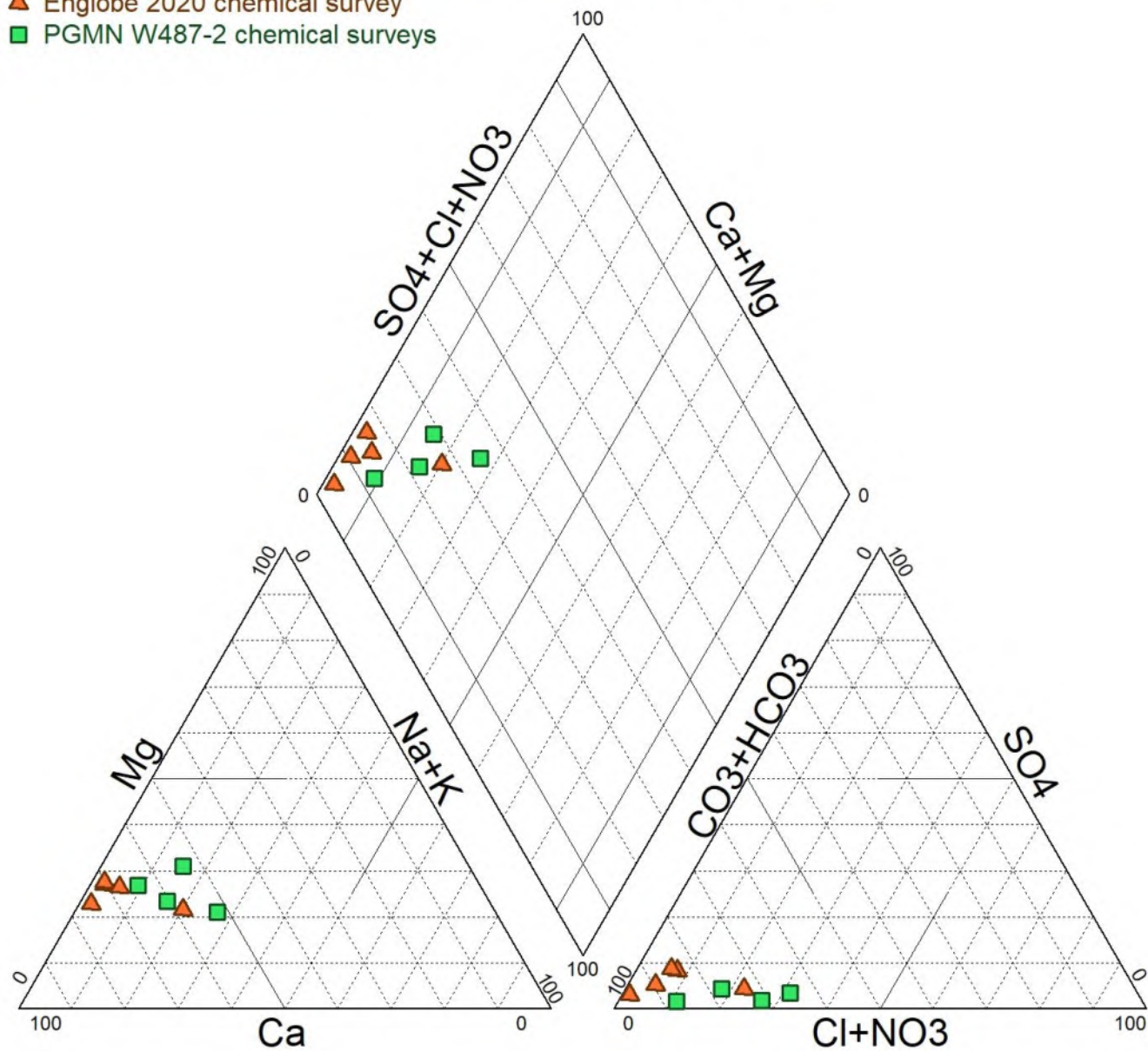
Figure 4: Piper Diagram
