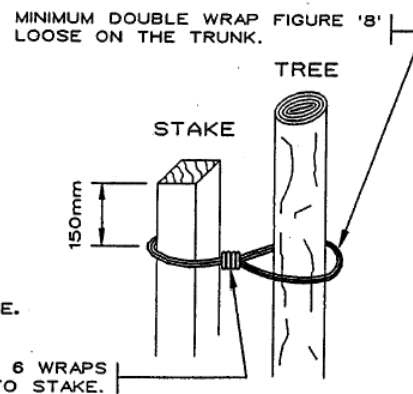
TWINE TIE DETAIL
