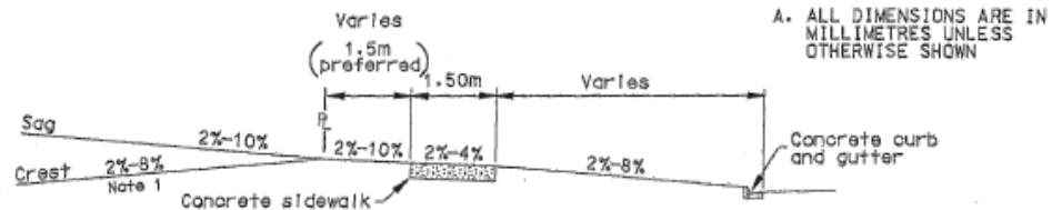
SECTION Z-Z FOR EXISTING R.O.W.s
