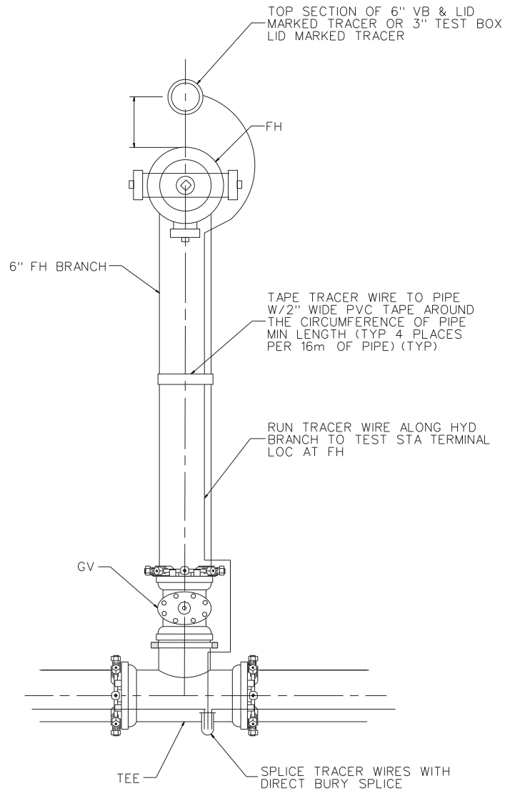
FIRE HYDRANT PLAN VIEW
